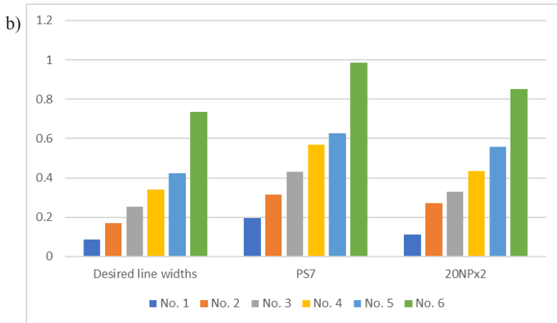
Figure 3. Line width on laboratory paper (in millimetres (mm)) made with 20% wheat pulp (2NP) coated with one layer of TiO 2 (20NPx1) and two layers of TiO 2 (20NPx2) in comparison with the reference sample (PS7)
